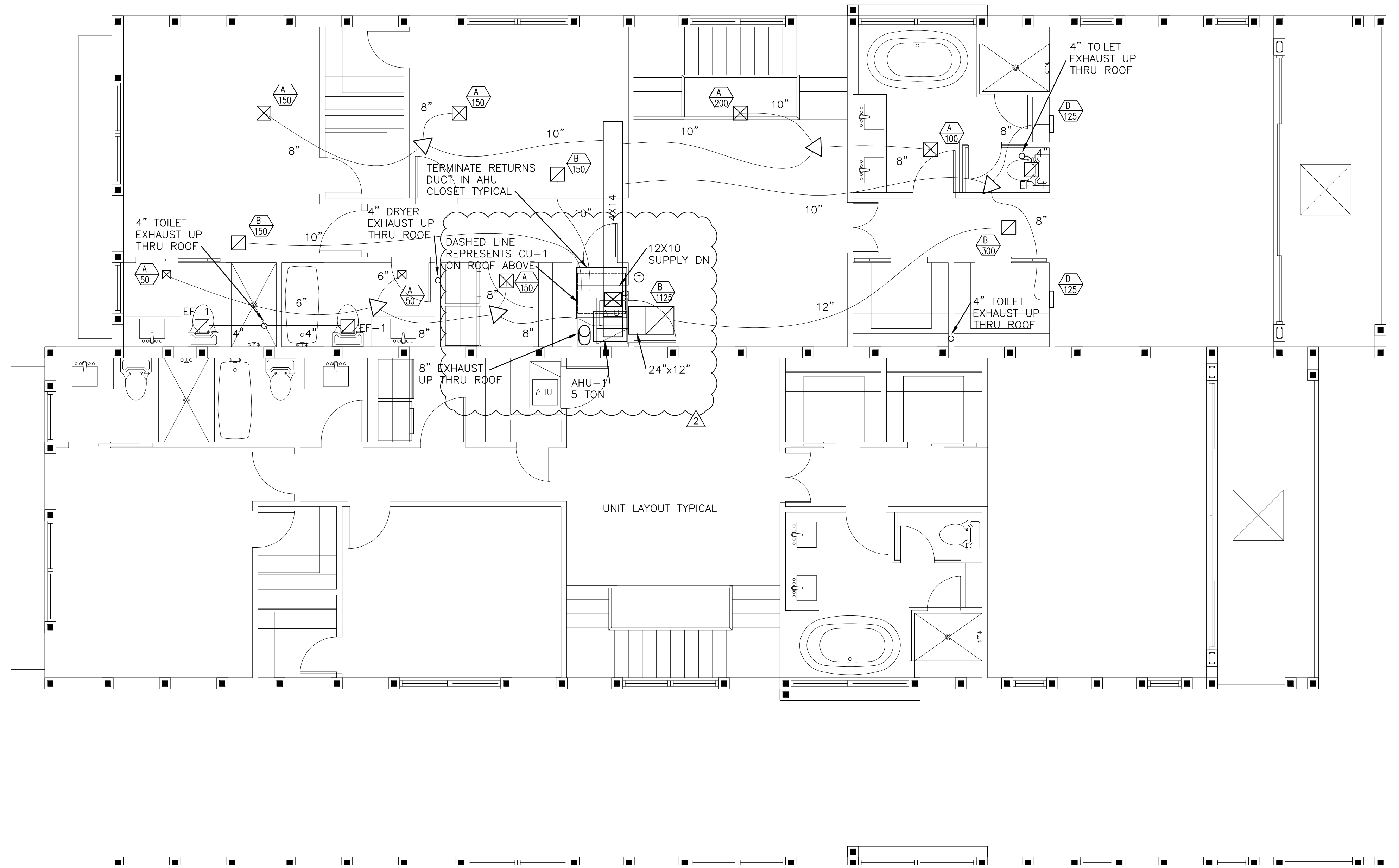
Mechanical Second Floor Plan Scale 1/4" = 1'-0"
