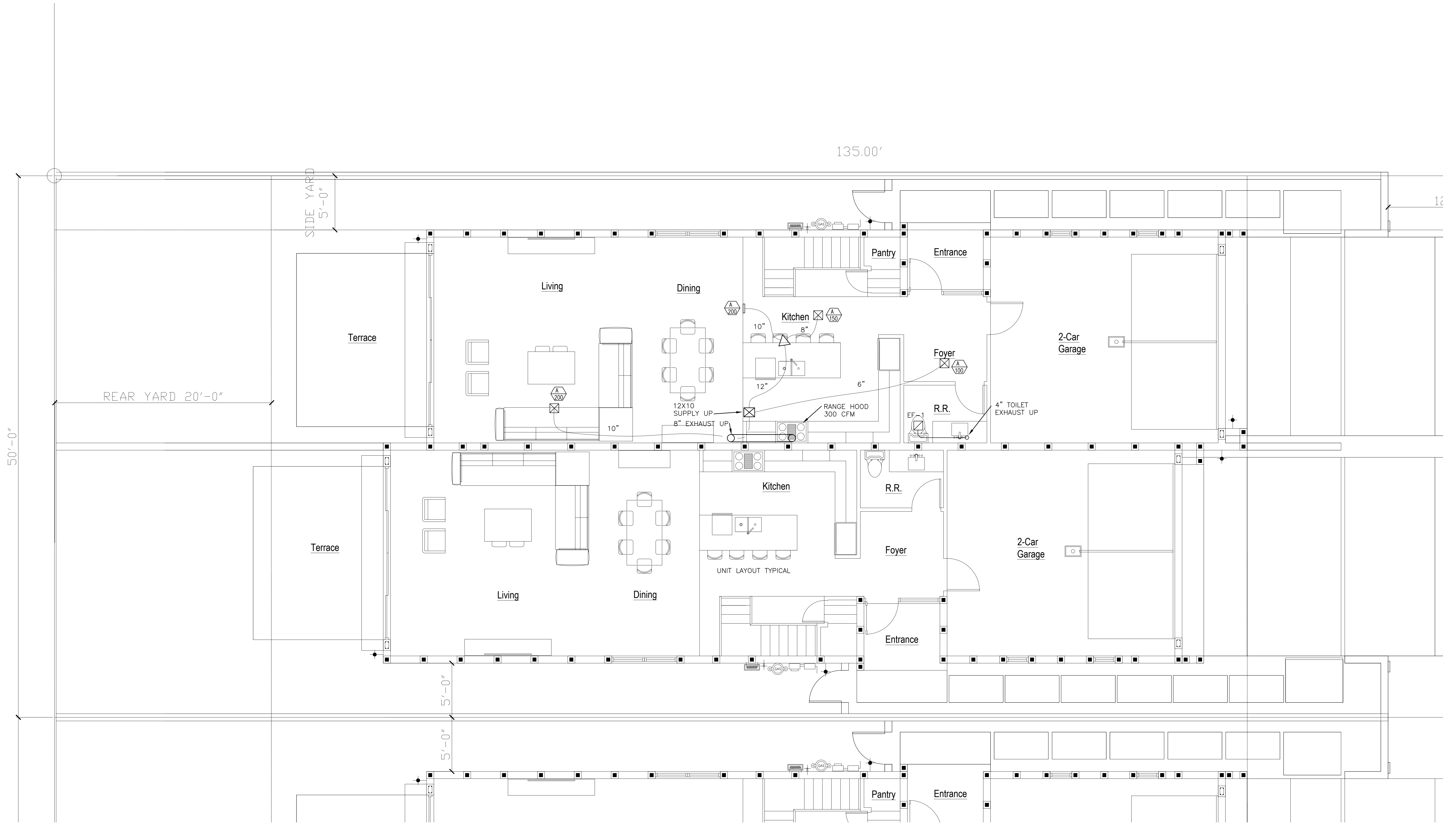
Mechanical First Floor Plan Scale 1/4" = 1'-0"
