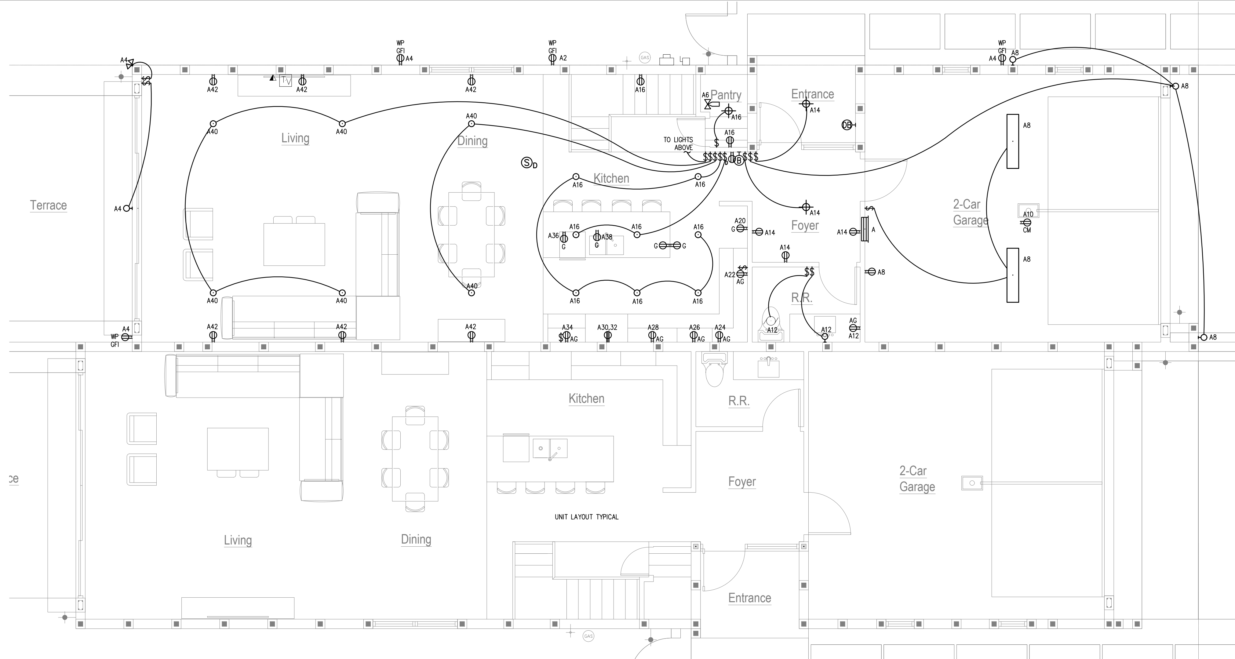
Electrical First Floor Plan Scale 1/4" = 1'-0"
